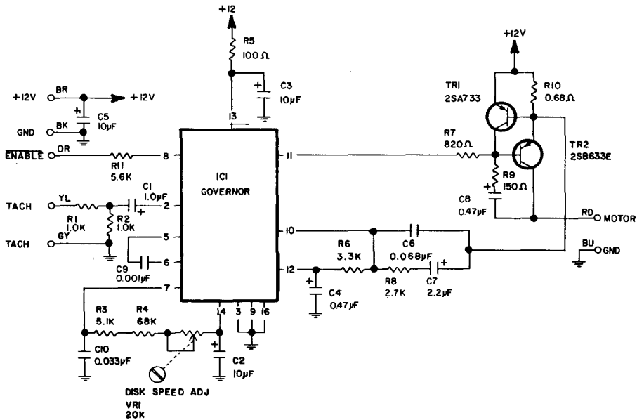
Fig. A-11. Drive motor servo circuit, Model 1542.
